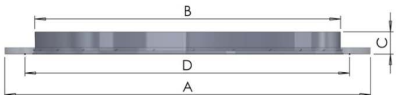
SSW-HC-16-C Circular Swirl Diffuser
