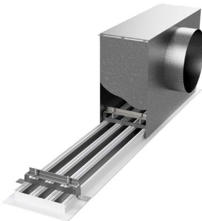
Folded for plasterboard ceiling
